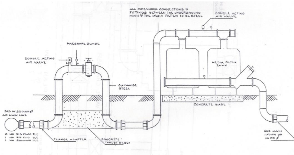
Fig 1: Sand Filter Assembly
