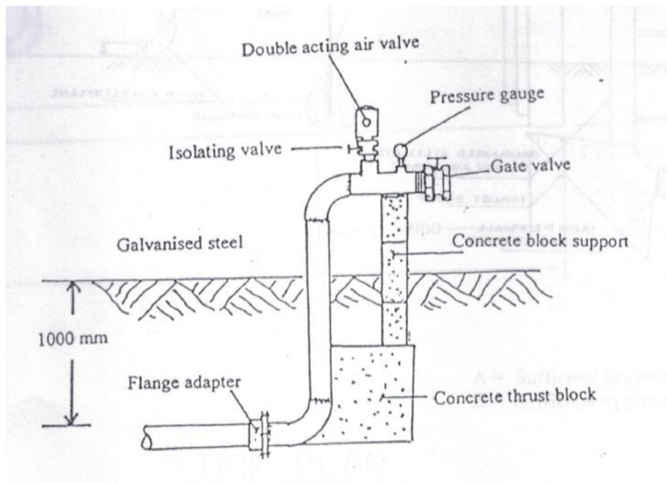
Fig 4: Drain/Air Valve Assembly
