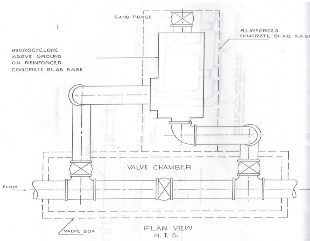
Fig 2: Hydrocyclone Assembly
